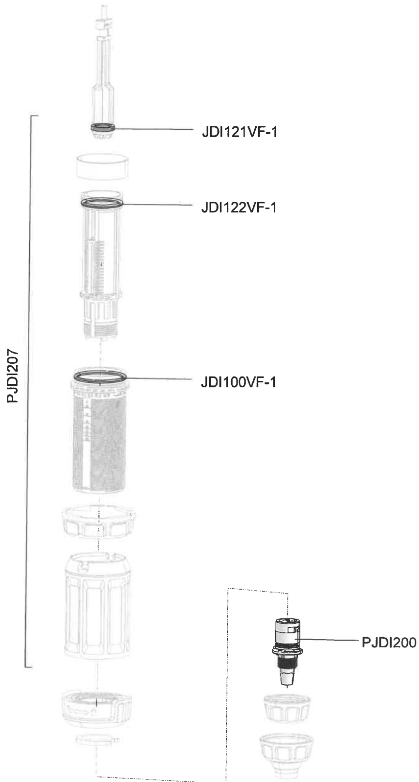
Seal Kit - PJD1207 (JDI121VF-1, JDI122VF-1, JDI100VF-1, PJD1200)
