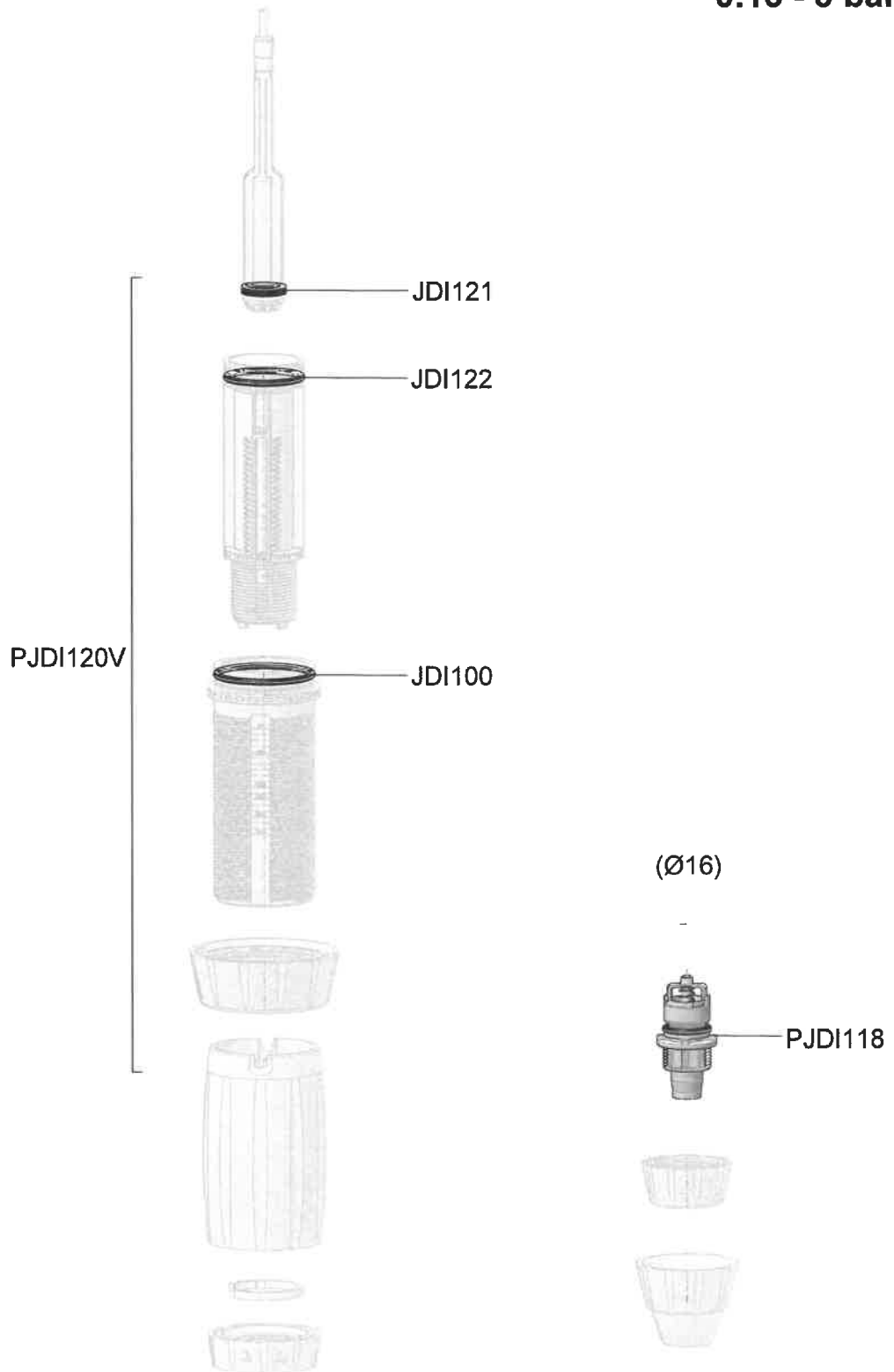
Seal Kit - PJD120V (JDI121, JDI122, JDI100, PJD118)
