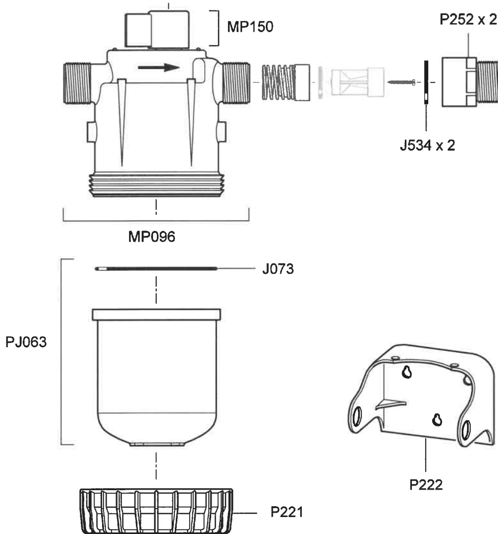
PVDF - MP096P - Upper Body Assembly PVDF Including MP150 PJ063P - Lower Body PVDF and Seal P221P - Body Connection Nut PVDF
