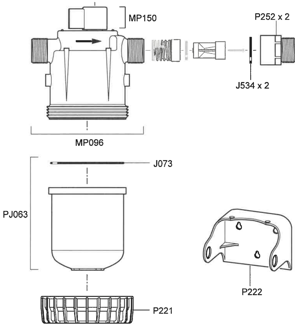
PVDF - MP096P - Upper Body Assembly PVDF Including MP150 PJ063P - Lower Body PVDF and Seal P221P - Body Connection Nut PVDF
