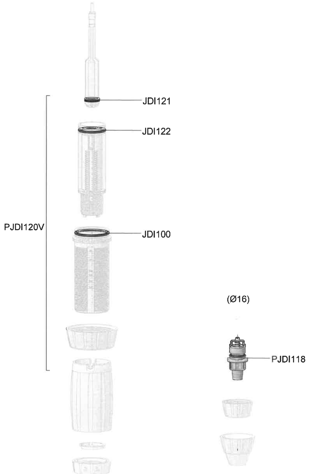
Seal Kit - PJD120V (JDI121, JDI122, JDI100, PJD1118)
