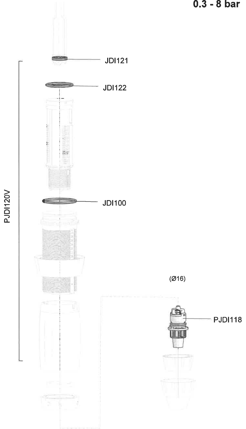
Seal Kit - PJD120V (JDI121, JDI122, JDI100, PJD118)
